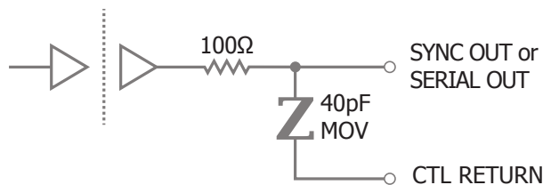
Figure 20: Internal circuitry for SYNC OUT and SERIAL OUT pins.
